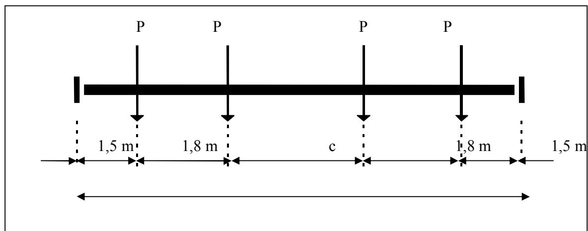
Limits for classification into track load classes
